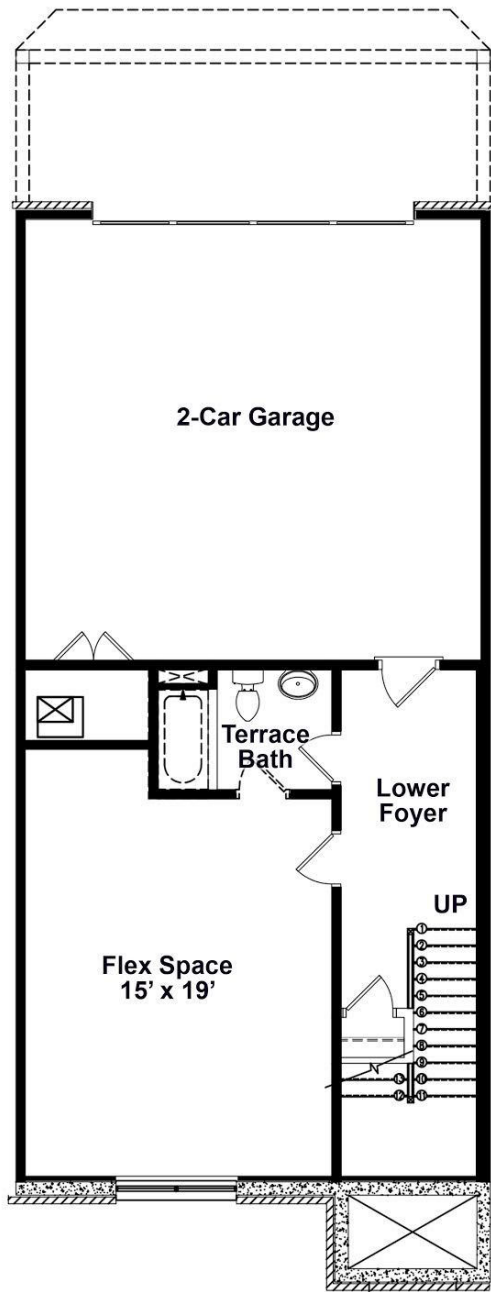
Lower Level Plan Option 1
