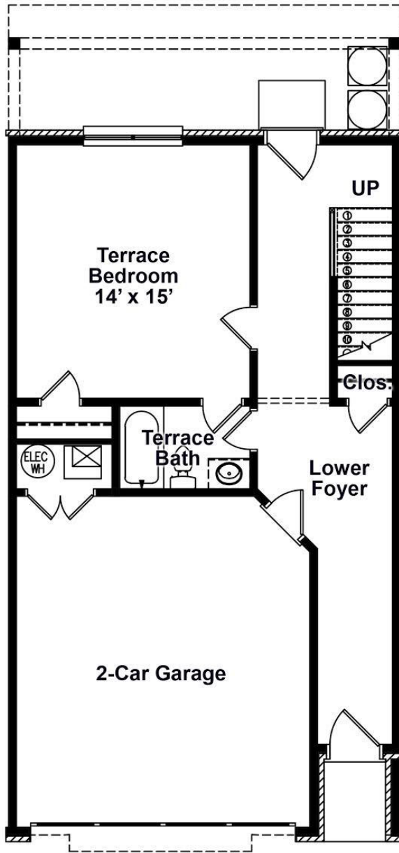
Lower Level Plan - Option 1
