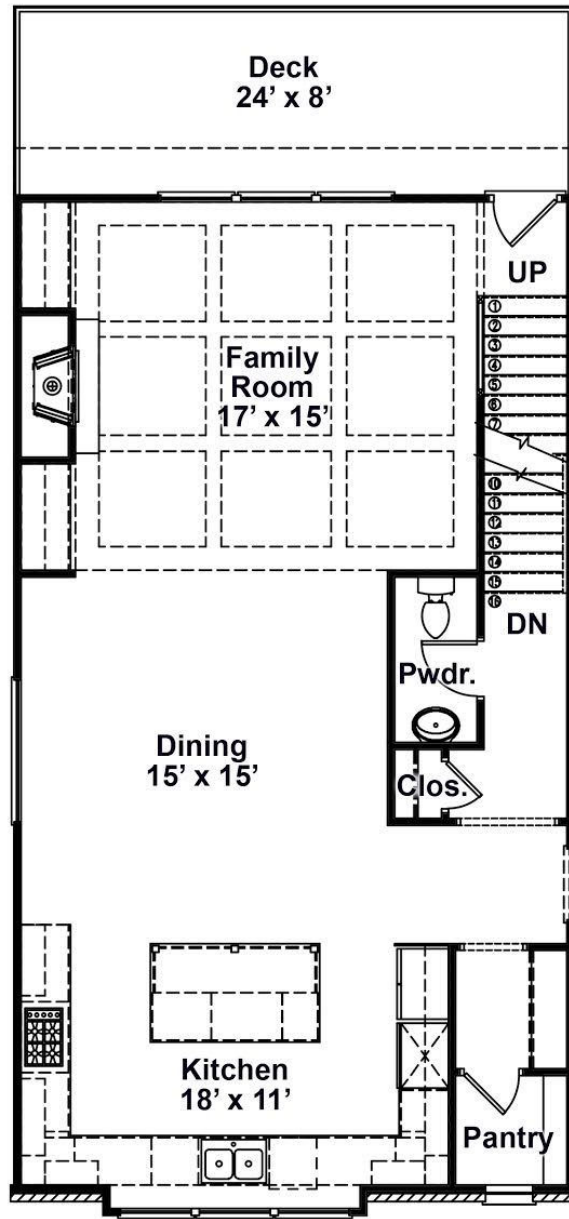
Main Level Plan
